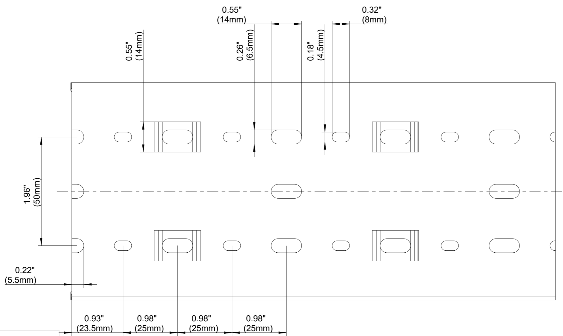
BASE PERFORATION
